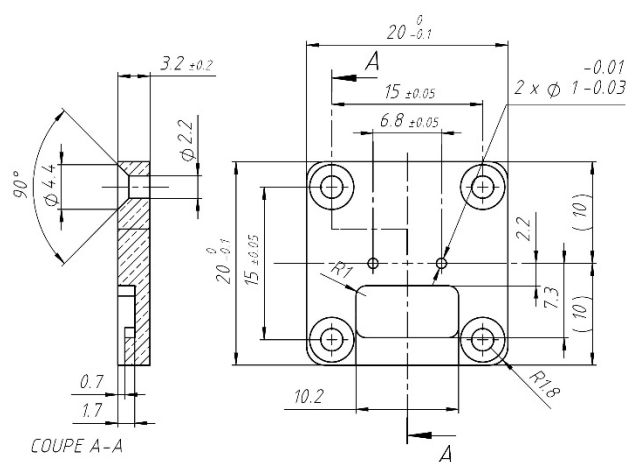
Fig. 5 Dimensions (mm) of encoder-holder type A.
