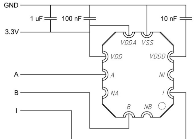
Fig. 6 Recommended schematic for 3.3 V operation without in-circuit OTP programming. Application of the 6.5 V OTP programming voltage will cause permanent damage when VDD and VDDA are short-circuited.
