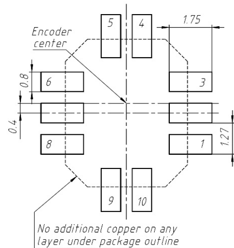
Fig 8 Recommended footprint.
