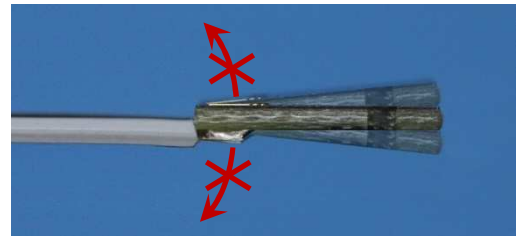
Fig. 3 Avoid bending of the solder joints.
